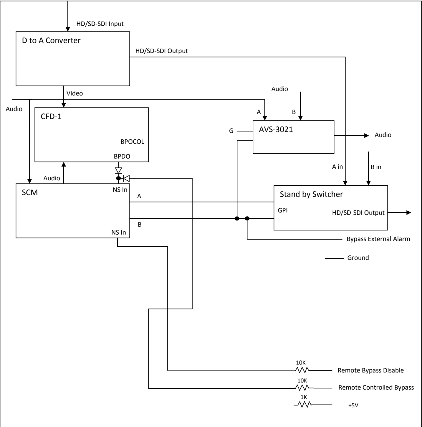
Spyglass HD/SD-SDI with Analog Audio Block Diagram
